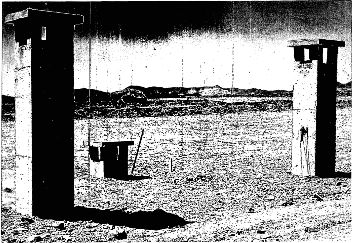
Fig. 7—Aboveground view of intake and exhaust stacks.
